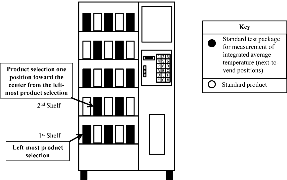
Figure A.1. Location of Standard Test Packages for Refrigerated Bottled or Canned Beverage Vending Machines with Products Arranged Horizontally and Five Next-to-Vend Product Locations on Each Shelf.
