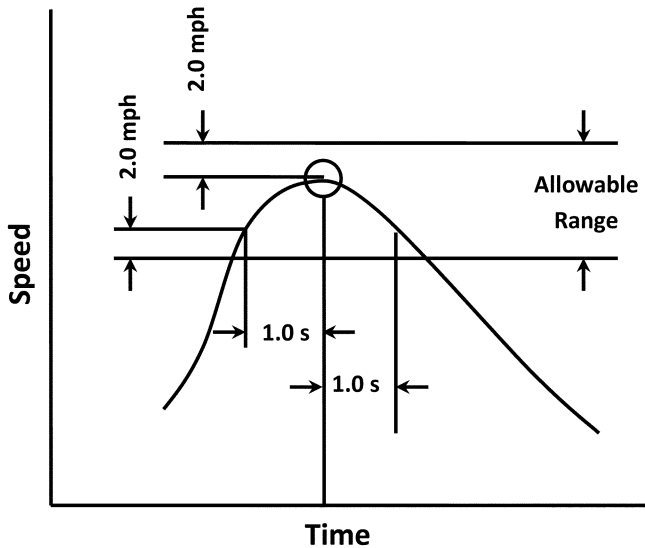
Figure 2 of § 1066.425—Example of the allowable ranges for the driver's trace
