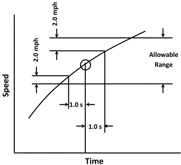
Figure 1 of § 1066.425—Example of the allowable ranges for the driver's trace
