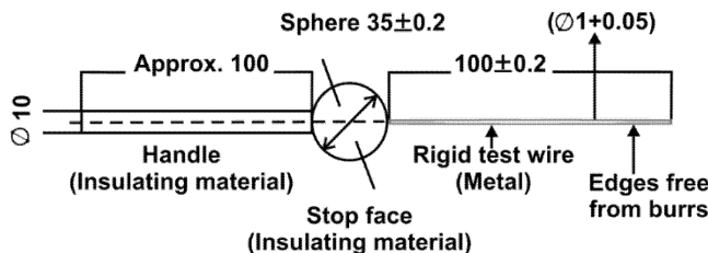
Figure 7a. S4, S5.3, S5.4.1.3, and S5.4.1.4 Access probes for the tests of direct contact protection. Access probe IPXXB (top) and Access probe IPXXD (bottom).
