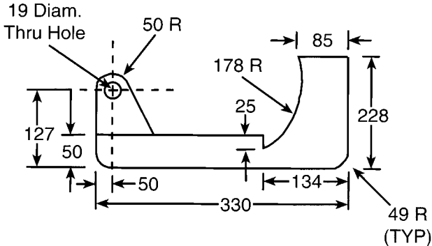
Figure 2B.—OPTIONAL BODY BLOCK FOR CENTER SEATING POSITIONS
