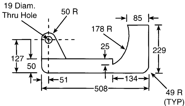
Figure 2A.—BODY BLOCK FOR LAP BELT ANCHORAGE
