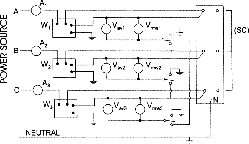
Figure 4.3 Three-Phase Test Set Without Instrument Transformers
