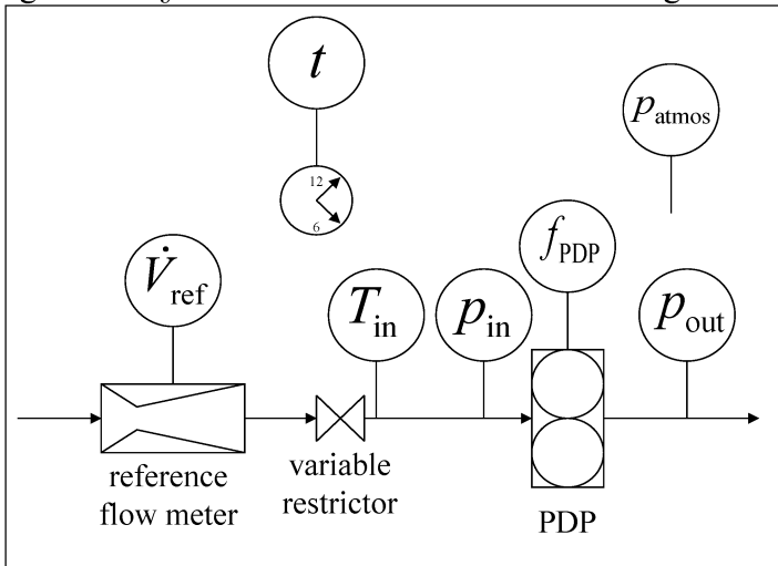
Figure 1 of § 1066.140—CVS calibration configurations
