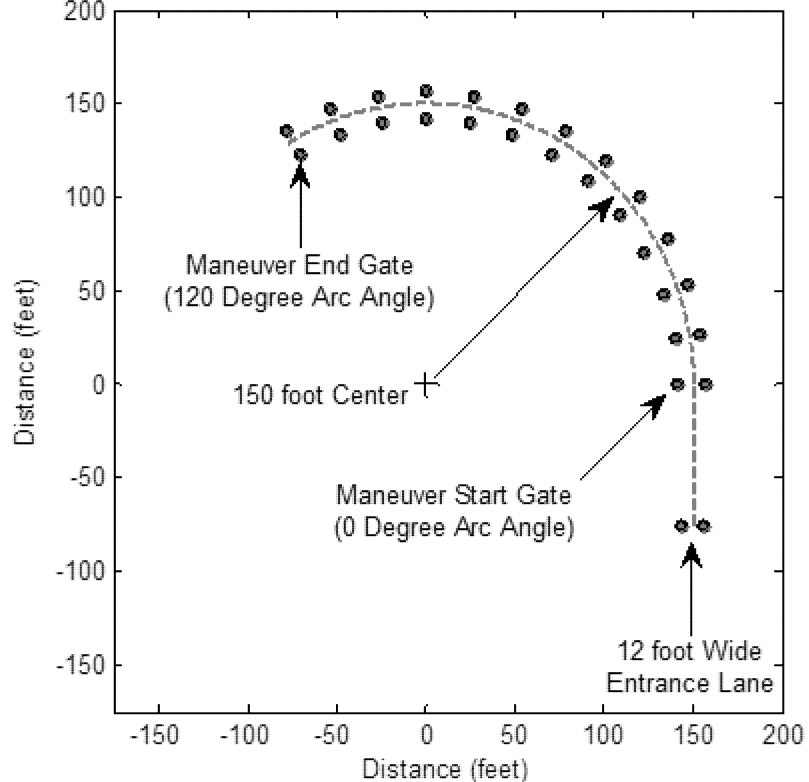
Figure 1. J-Turn Test Maneuver Course (shown with the curved lane section in the counter-clockwise direction)
