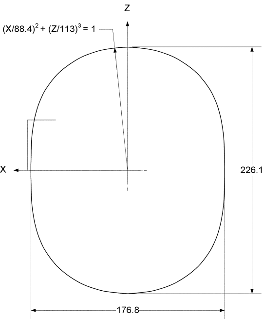
Figure 1 – Ejection Headform Face. All dimensions are millimeters.
