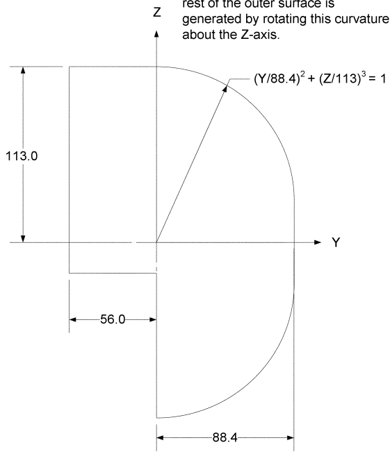
Figure 1 – Ejection Headform Face. All dimensions are millimeters.
