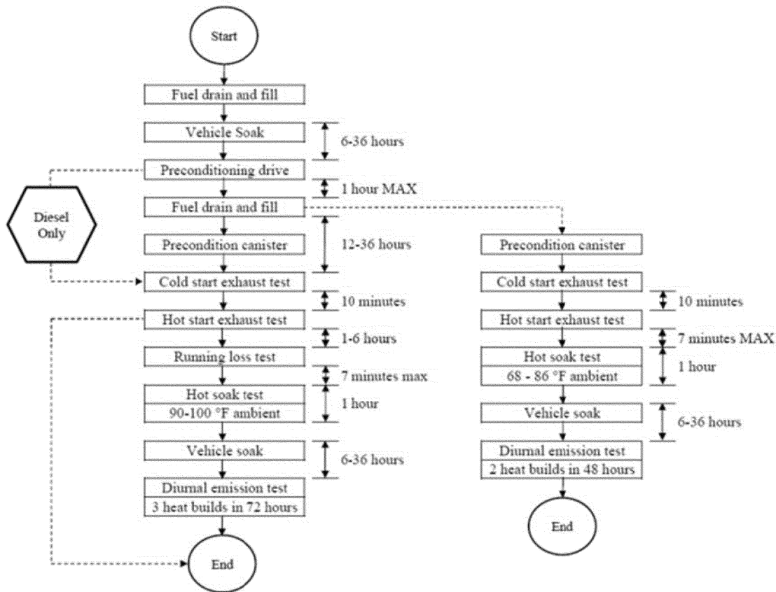
Figure 1 of §1066.801 —FTP test sequence
