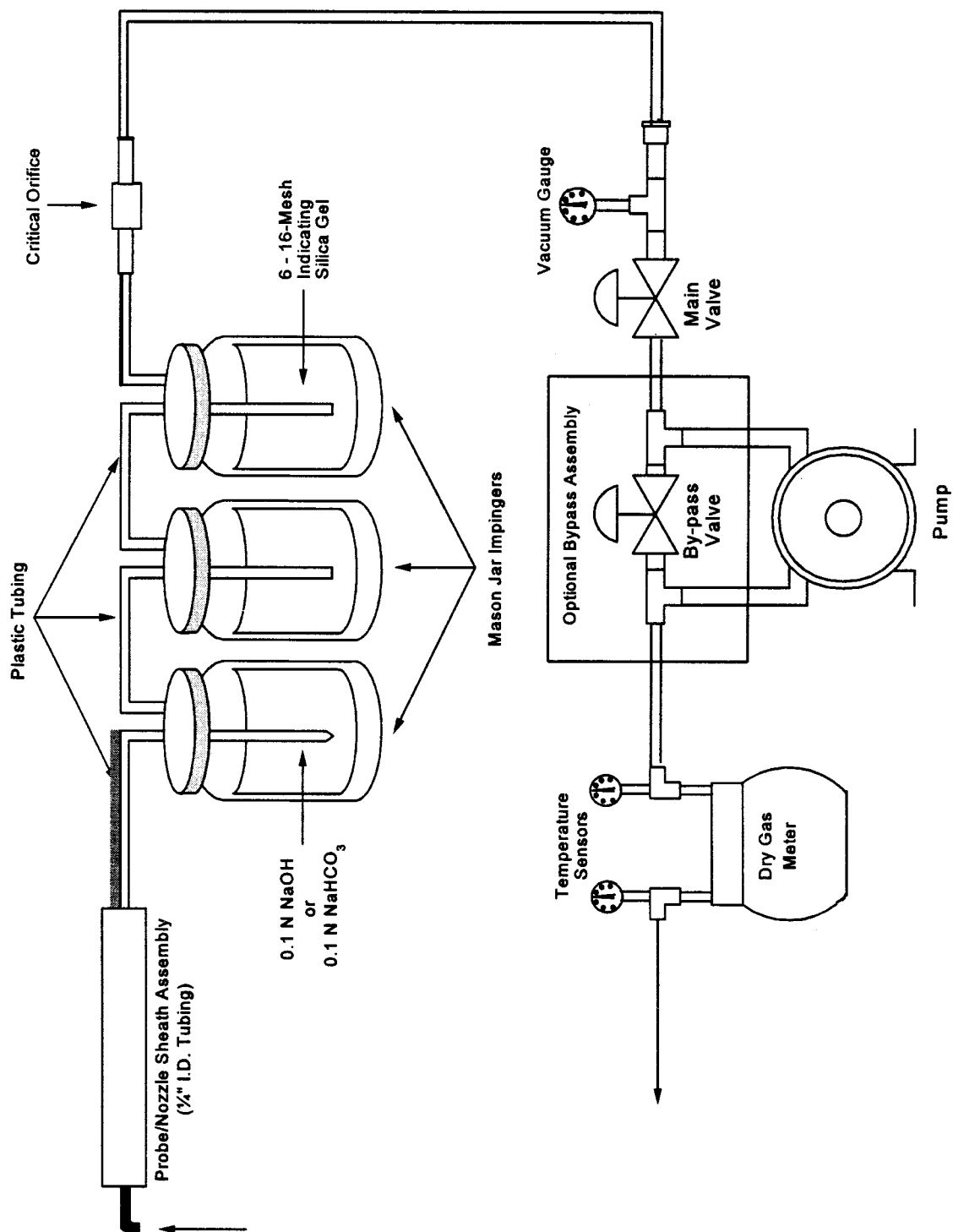
Figure 306A-1. Method 306A Sampling Train.
