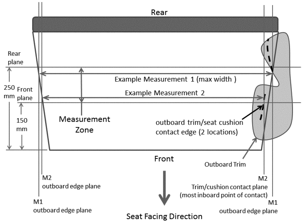
FIGURE 1: Example Measurements for Seat Cushion Width
