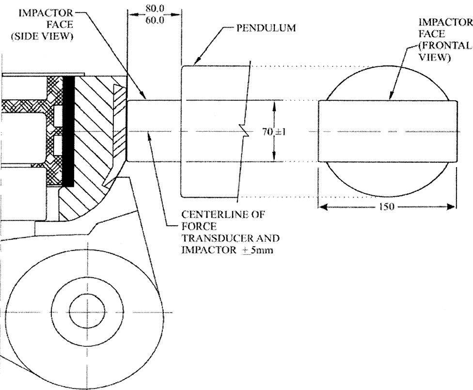
ABDOMEN TEST SET-UP
