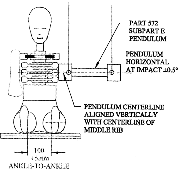
Figure U4 THORAX IMPACT
