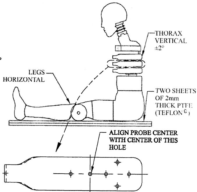
RIB DETAIL (REF. DWG. 175-4004)
