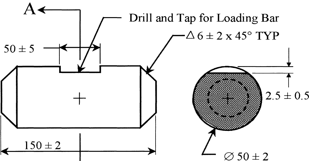
Figure A1 to Appendix A and Appendix A-1 of FMVSS No. 208 Regulatory Text: Loading Bar Foot Detail
