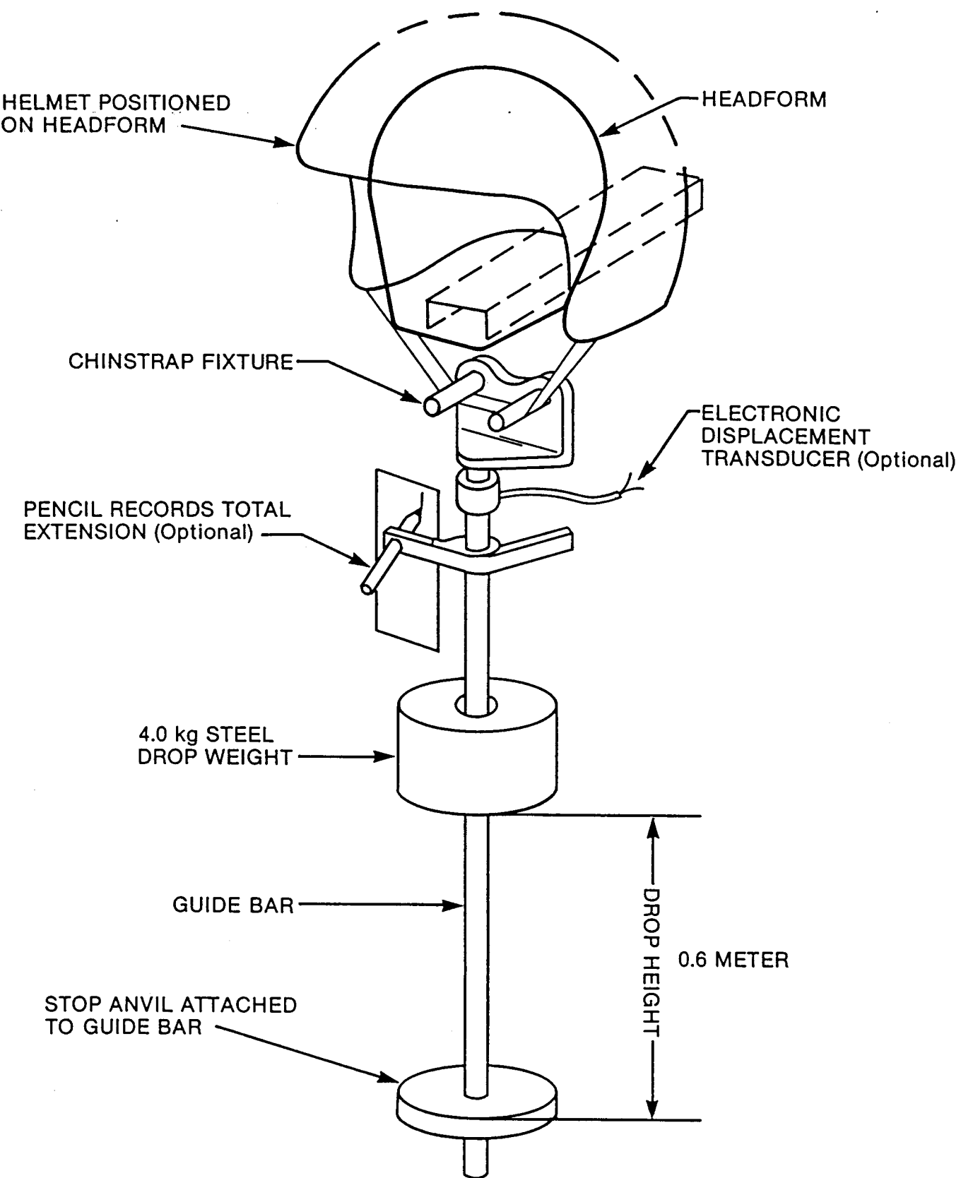
Figure 8. Apparatus for Test of Retention System Strength
