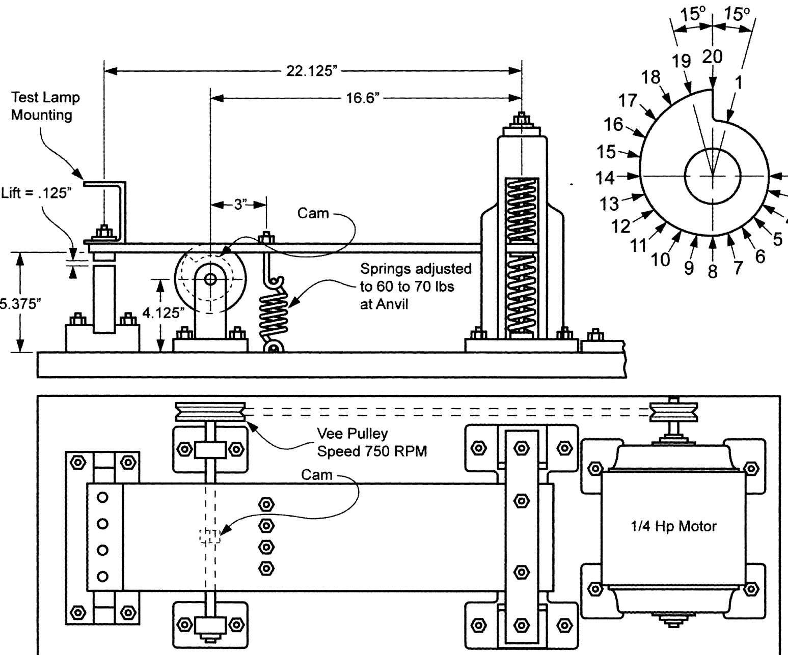
FIGURE 21 VIBRATION TEST MACHINE
