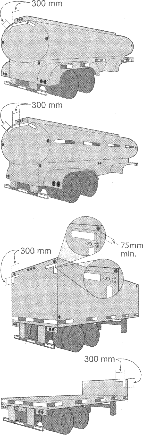
Trailer Conspicuity Treatment Examples
