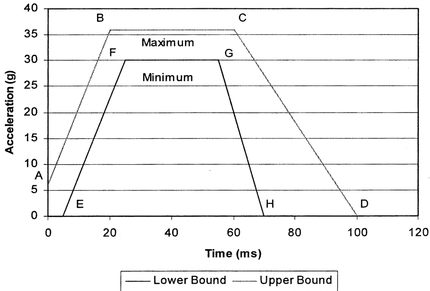
FIGURE 6 – ACCELERATION PULSE
