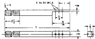
GUIDE ROD 1 REQ. ALUM.
