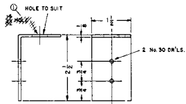
FUEL VALVE BRACKET 1 REQ. ALUM.
