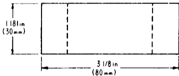
FIG 1-RATTLE TEST FIXTURE
