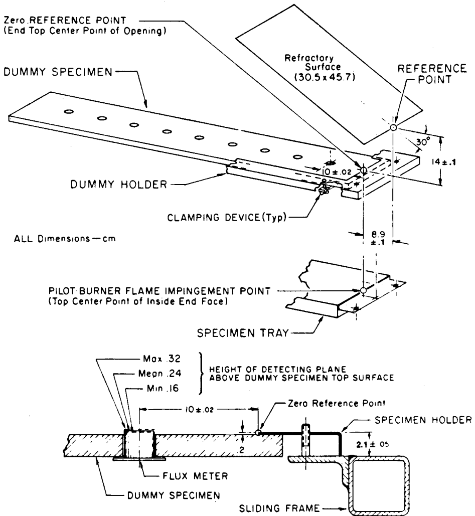
FIG 5 — ZERO REFERENCE POINT RELATED TO DETECTING PLANE
