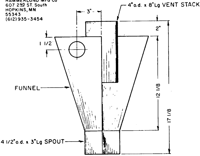
FIG 2—CYCLONE RECEIVER WELDMENT
