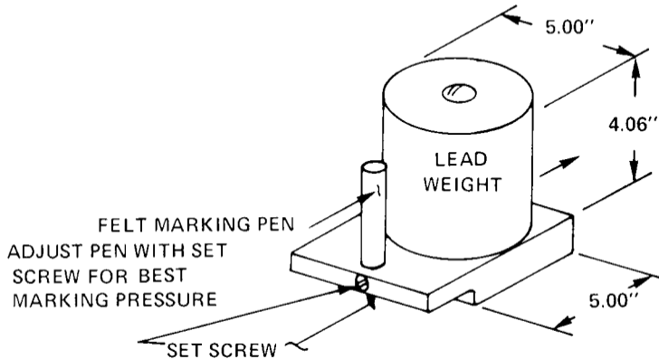
FIG. G ASSEMBLY FOR MEASUREMENT OF RUNWAY EQUILIBRIUM
