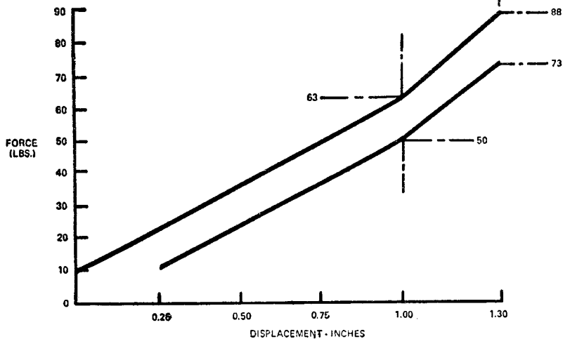
FIGURE NO. 10 ABDOMEN COMPONENT TEST
