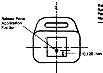
7c. Hinged Button
