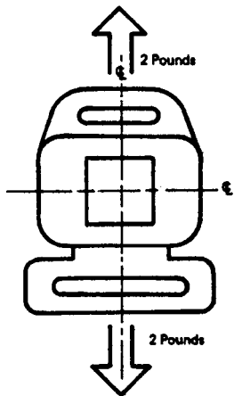
7a. Single Latch Plate Pre-load
