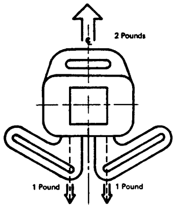
7b. Double Latch Plate Pre-load
